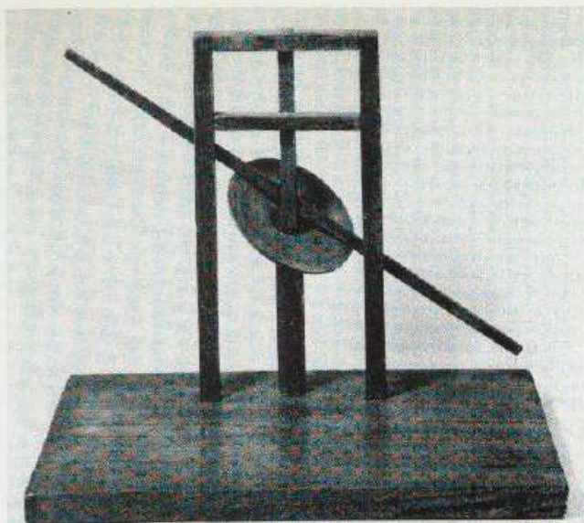
How a disc fastened to a vertical axis transforms its rotary movement to the pumping of an attached arm. 13\frac{1}{4} " high \times 15" long \times 9" deep
