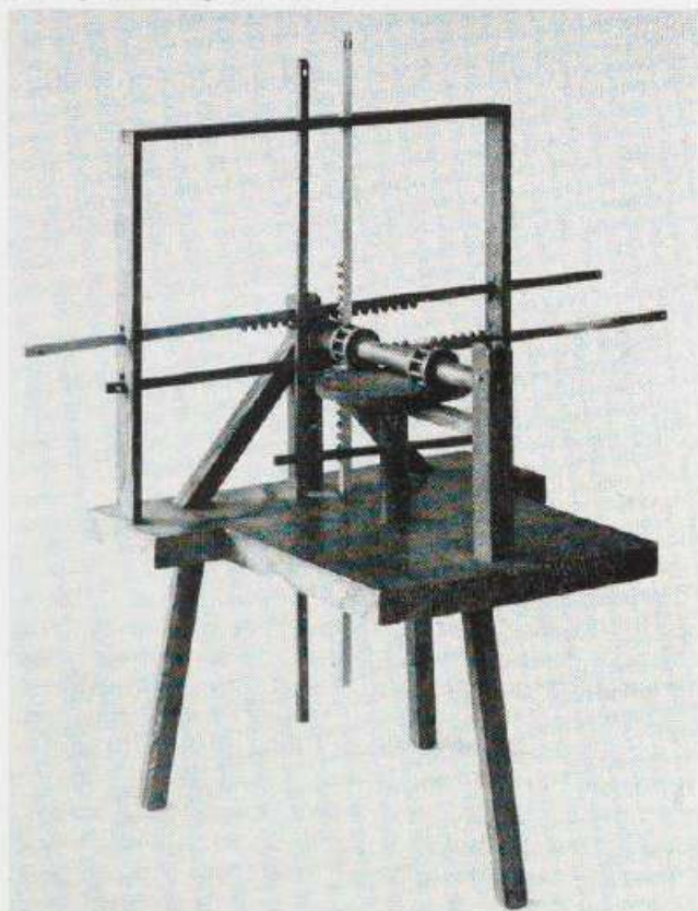
How rotary movement transforms the action of 4 straight rods (2 vertical, 2 horizontal) into reciprocating motion. 20\frac{1}{4} " high \times 17" long \times 11" deep
