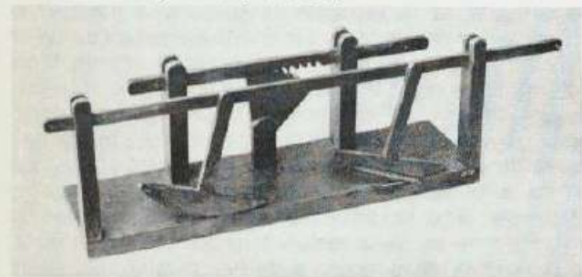
Three ways to lift and steer a rod making a straight reversible movement. 7\frac{1}{2} " high \times 26" long \times 5" deep
