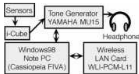
Fig. 10 Construction of prototype CosTune.
