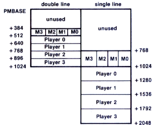
Figure 4-2 Player-Missile RAM Area Layout
