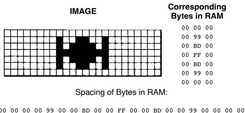
Figure 4-1 Noncontiguous RAM Images
