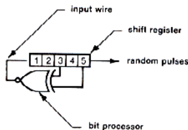
Figure 7-4 5-Bit Poly-Counter
