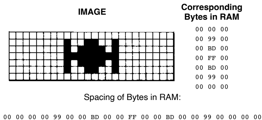
Image Bytes Scattered Through RAM
