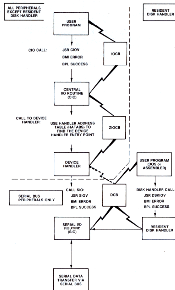
Figure 8-8 I/O Subsystem
