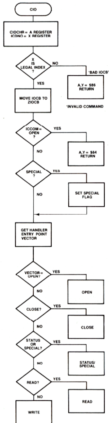
Figure 8-11.1 CIO Routine
