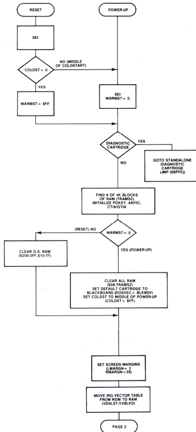
Figure 8-1.1 System Initialization
