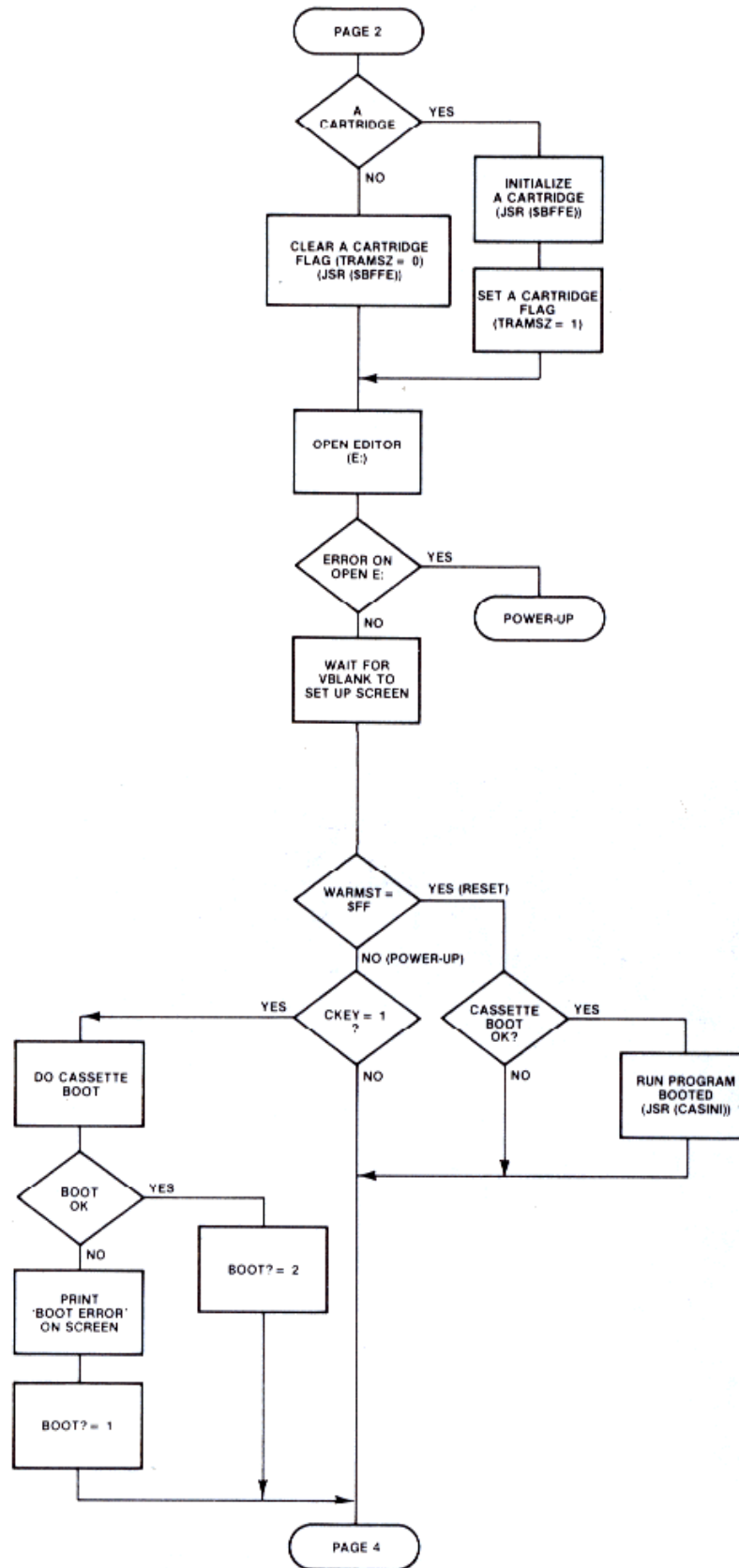
Figure 8-1.3 System Initialization
