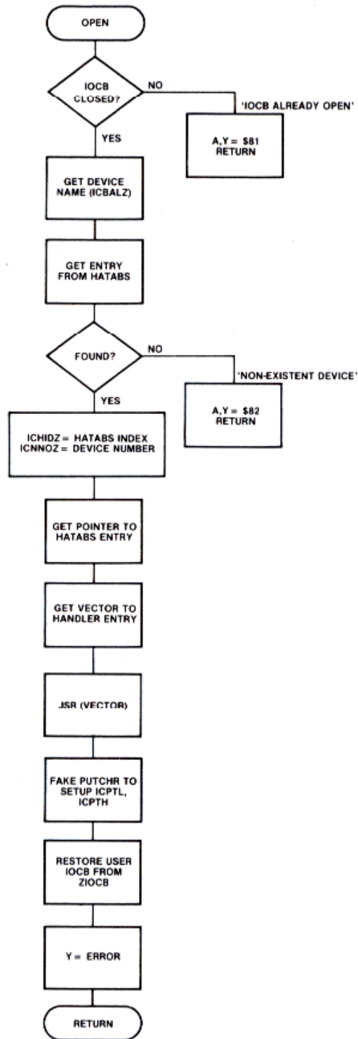
Figure 8-11.2 CIO Routine
