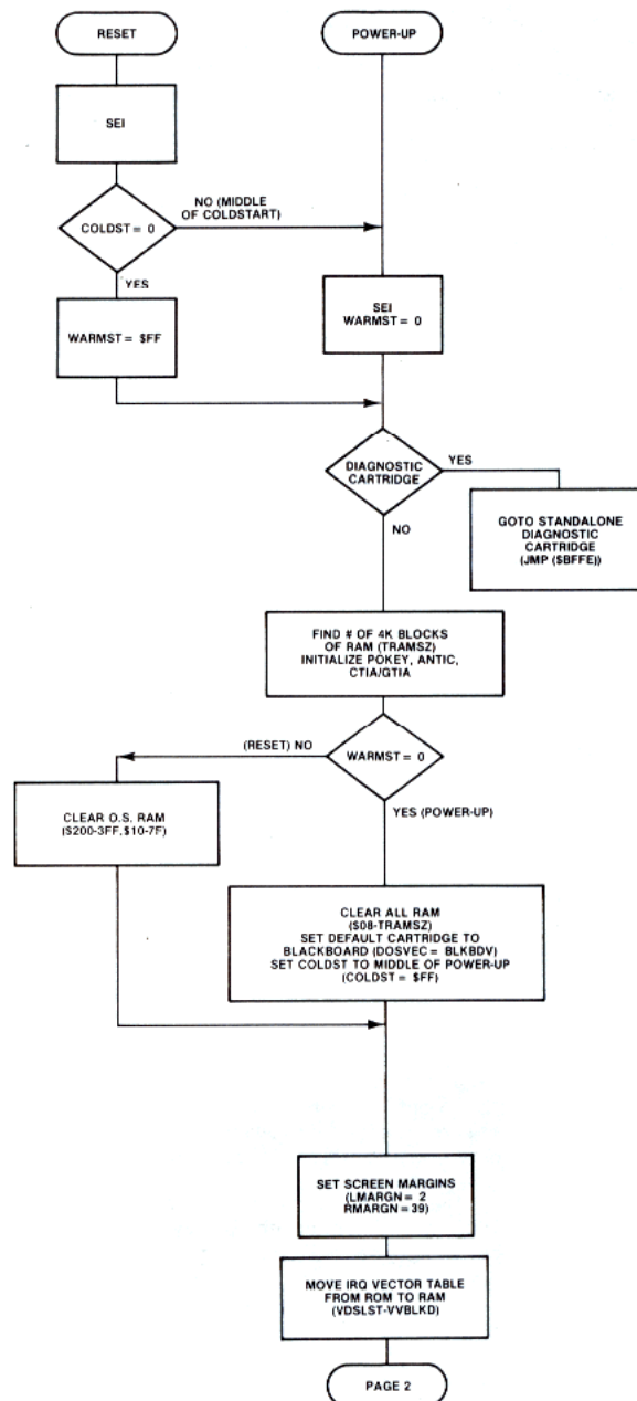
Figure 8-1.1 System Initialization
