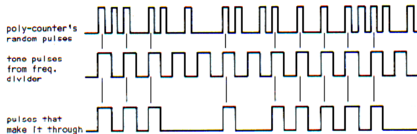
Figure 7-5 Selection Function Used To Mix In Distortion
