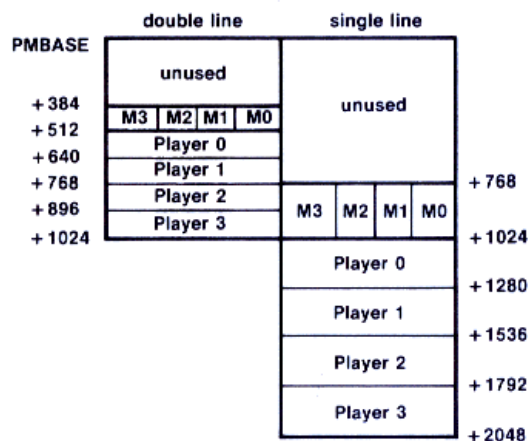
Figure 4-2 Player-Missile RAM Area Layout
