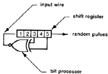
Figure 7-4 5-Bit Poly-Counter
