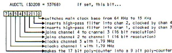
Figure 7-9 AUDCTL Bit Assignment
