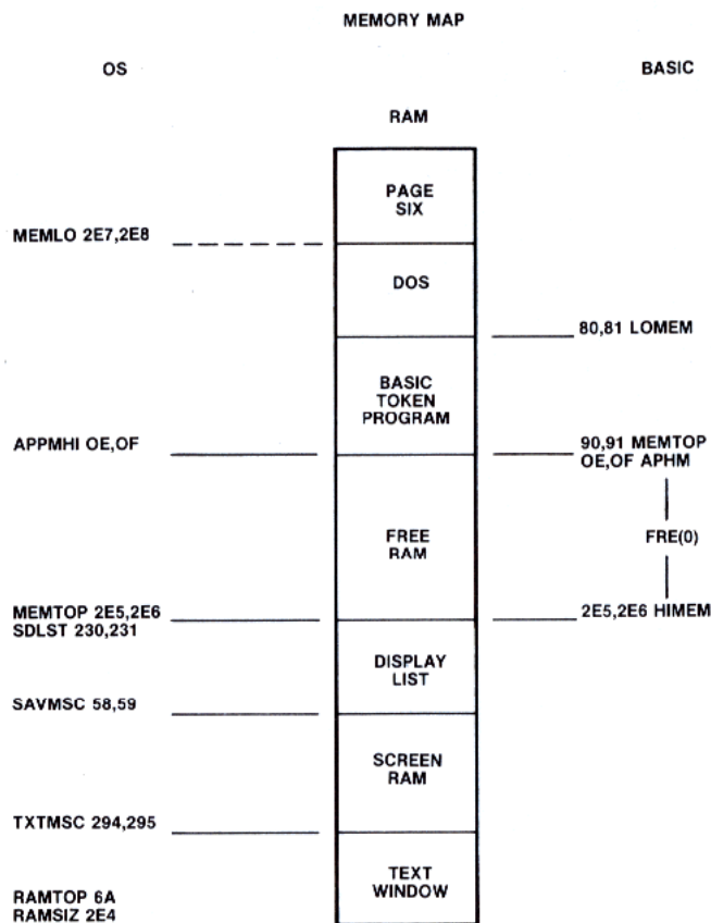
Figure 8-2 OS and BASIC Pointers (DOS present)
