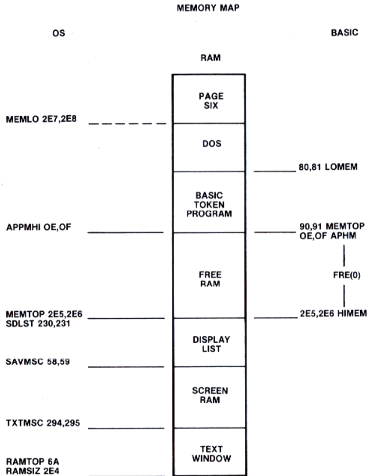
Figure 8-2 OS and BASIC Pointers (DOS present)
