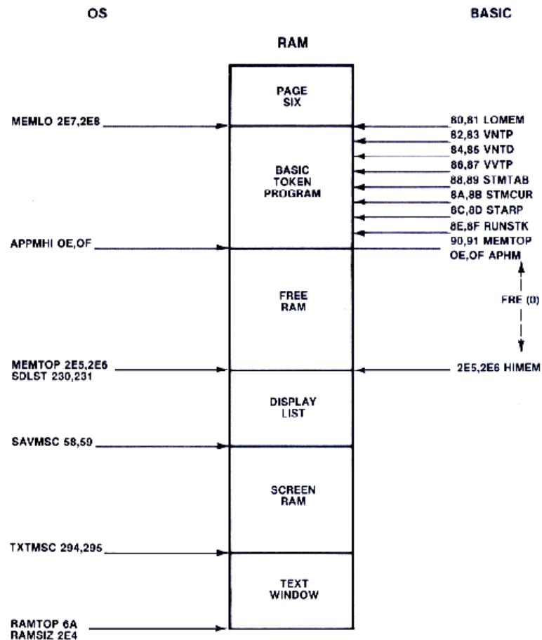
Figure 10-2 OS and BASIC Pointers (No DOS Present)
