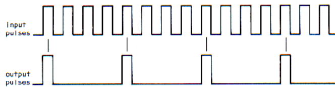
Figure 7-2 Divide-by-4 Operation
