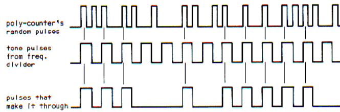
Figure 7-5 Selection Function Used To Mix In Distortion
