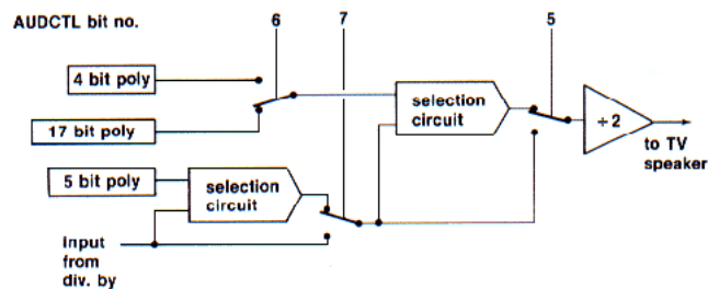
Figure 7-7 AUDC1-4 Block Diagram
