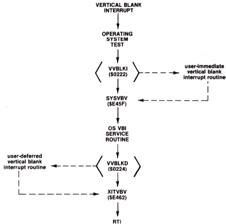
Figure 8-5 Vertical Blank Interrupt Execution
