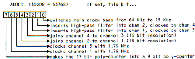
Figure 7-9 AUDCTL Bit Assignment
