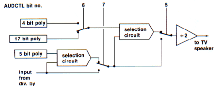
Figure 7-7 AUDC1-4 Block Diagram
