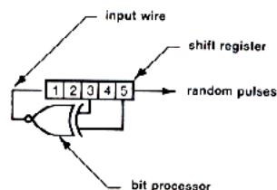
Figure 7-4 5-Bit Poly-Counter
