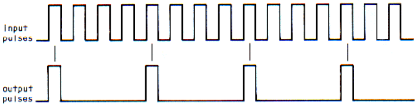
Figure 7-2 Divide-by-4 Operation
