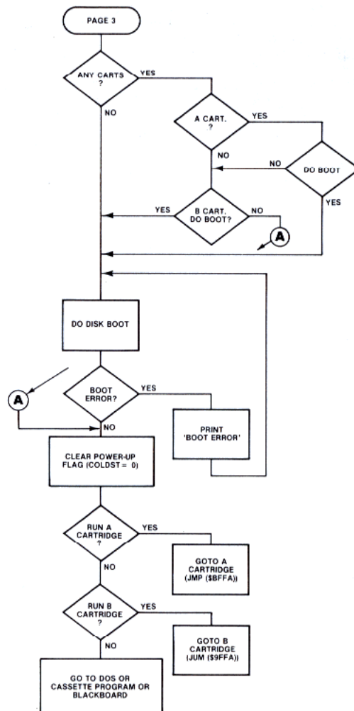
Figure 8-1.4 System Initialization
