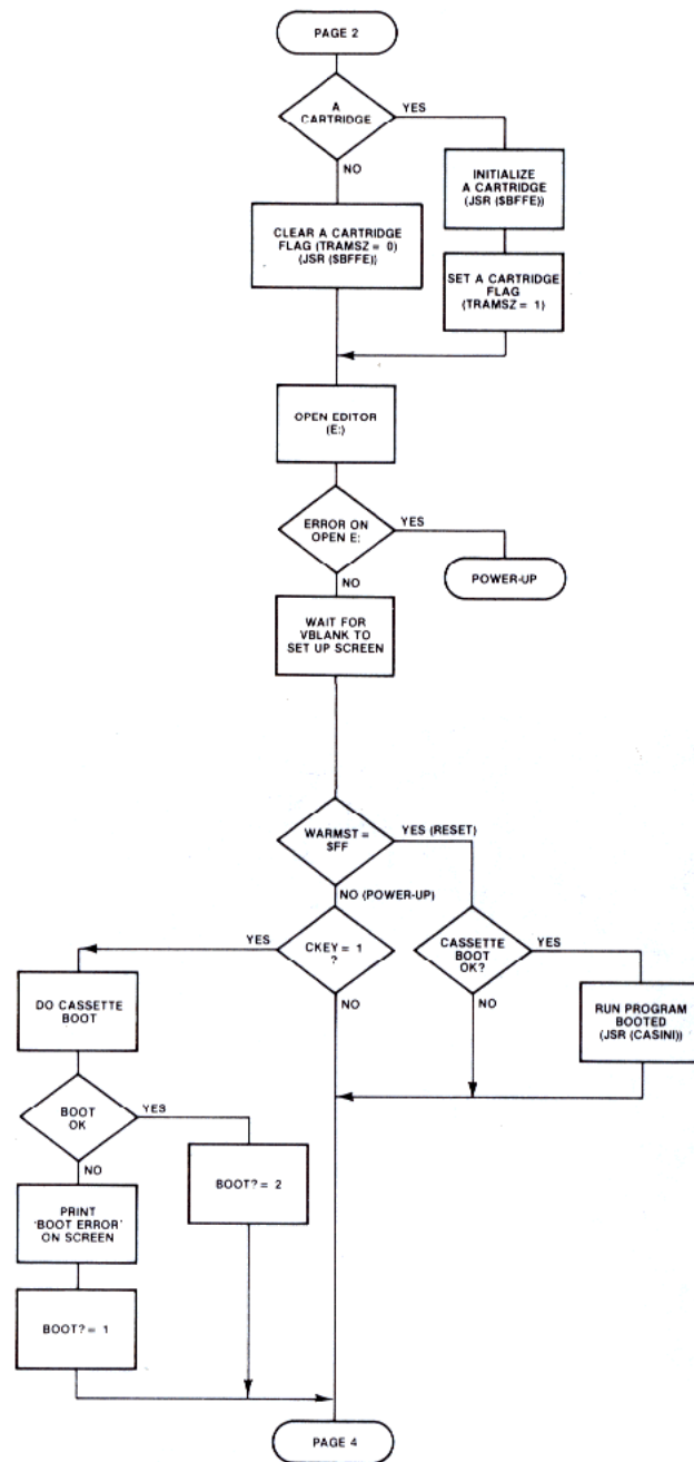
Figure 8-1.3 System Initialization
