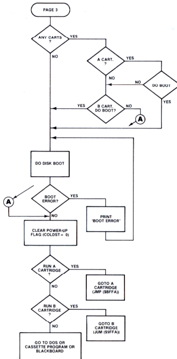
Figure 8-1.4 System Initialization
