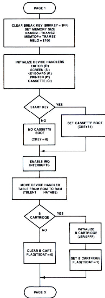
Figure 8-1.2 System Initialization
