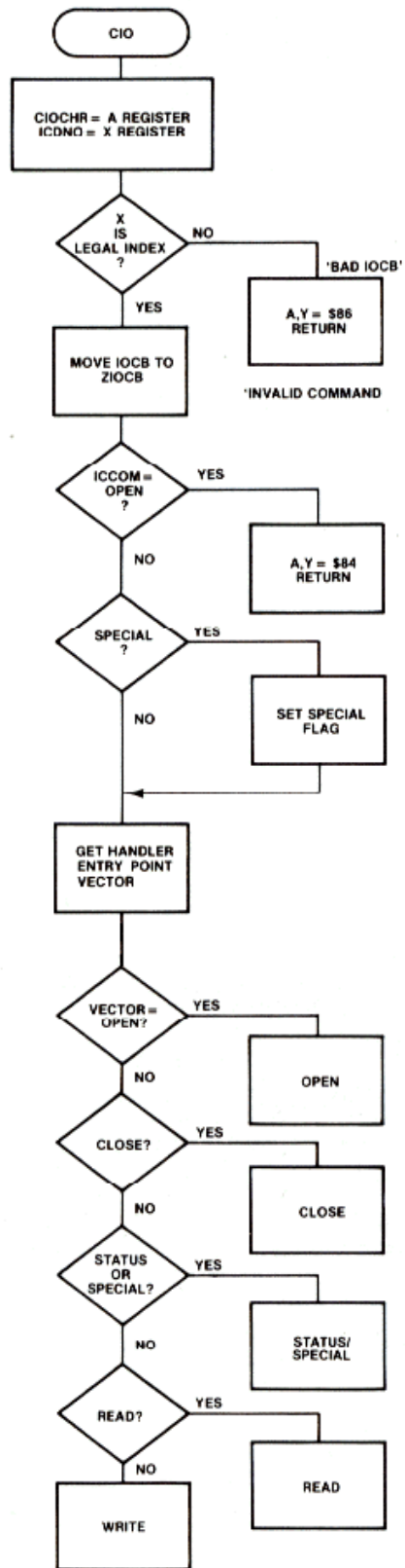
Figure 8-11.1 CIO Routine
