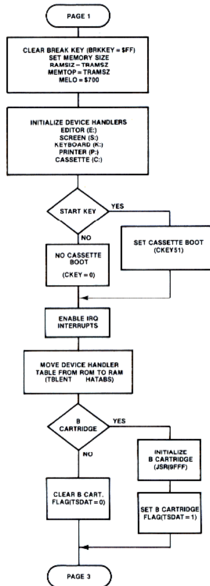
Figure 8-1.2 System Initialization
