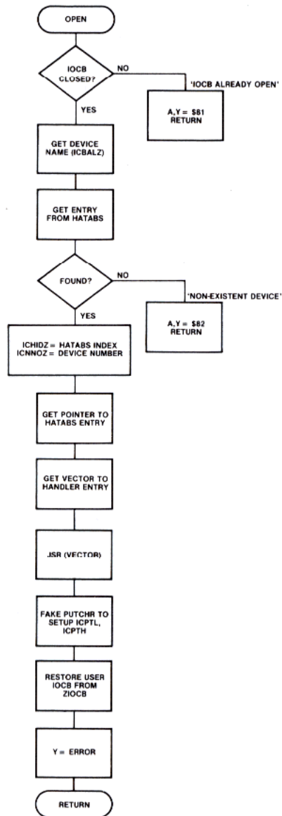
Figure 8-11.2 CIO Routine
