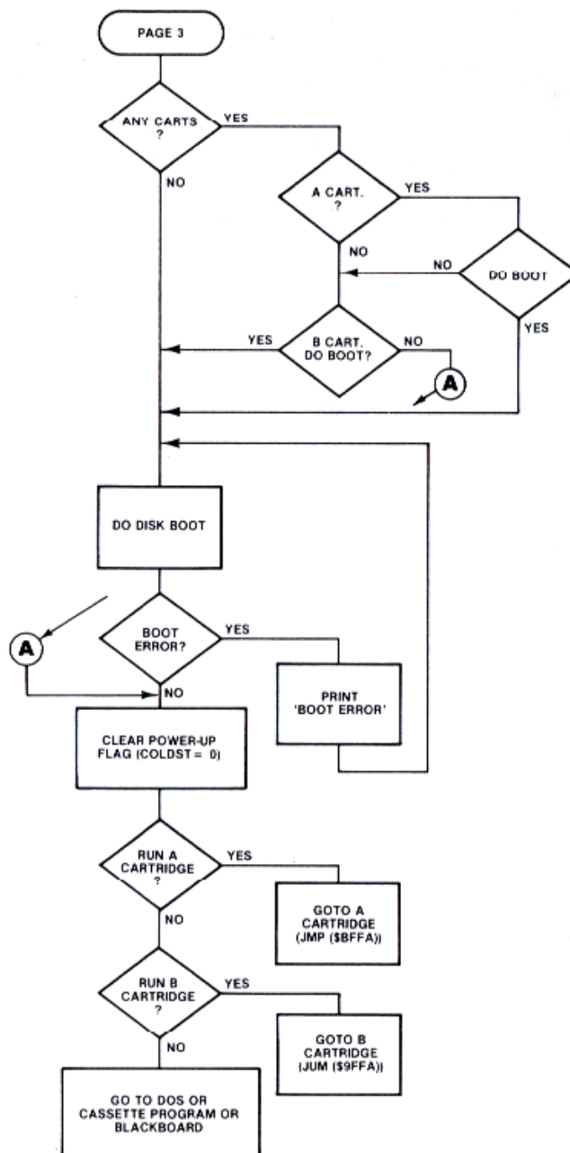
Figure 8-1.4 System Initialization
