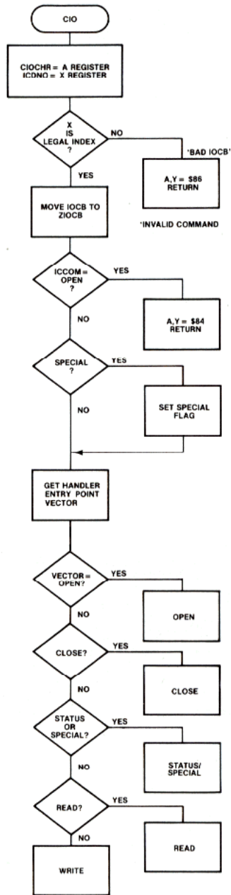
Figure 8-11.1 CIO Routine
