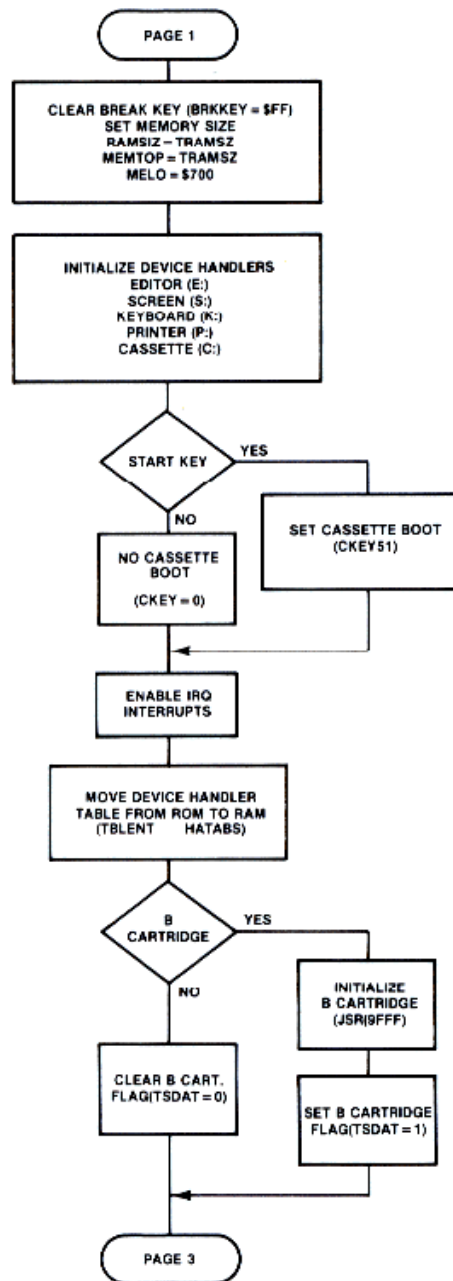
Figure 8-1.2 System Initialization
