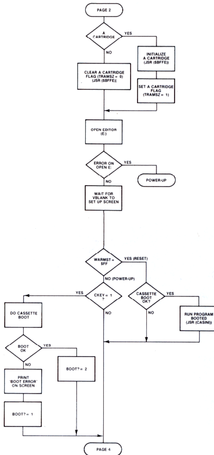
Figure 8-1.3 System Initialization
