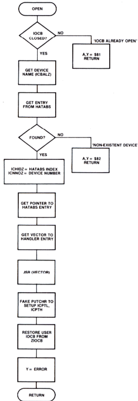
Figure 8-11.2 CIO Routine
