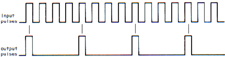
Figure 7-2 Divide-by-4 Operation
