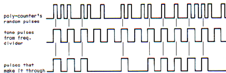
Figure 7-5 Selection Function Used To Mix In Distortion
