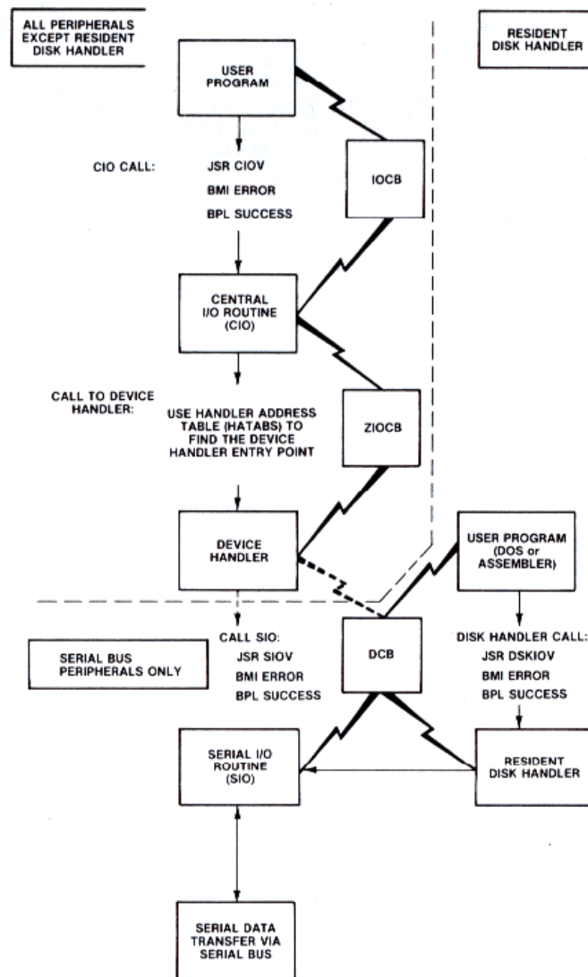
Figure 8-8 I/O Subsystem
