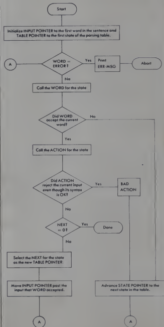
Figure 1. Flow chart for introductory automaton.
