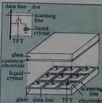
Figure 6. In TFT LCDs, each pixel has a corresponding thin film transistor deposited on one glass surface.
