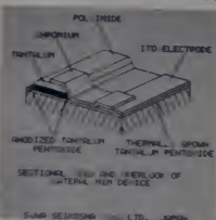
Figure 5. Experimental MIM LCD has 240 x 250 pixel matrix.
