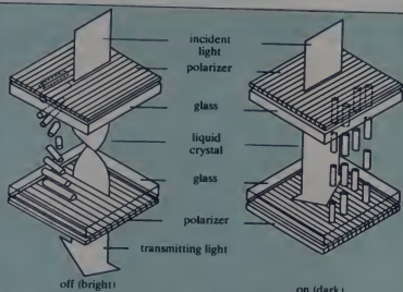
Figure 1. Principal of operation of twisted-nematic (TN) LCD.
