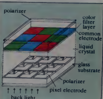
Figure 7. Structure of a full color TFT LCD.
