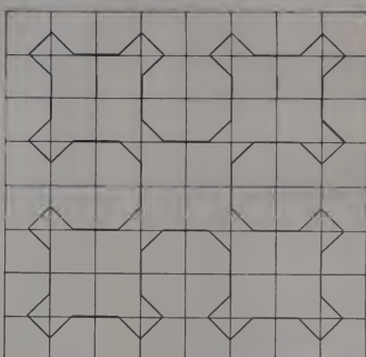
Figure 2. Construction of second order curve.
