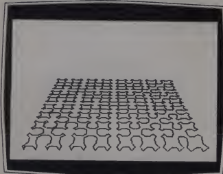
Figure 12. Tilted fourth order curve with straight sides.
