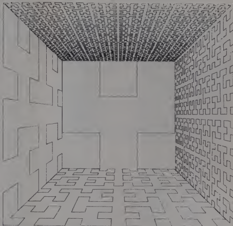
Cube made of Hilberts with orders 2 through 6.
