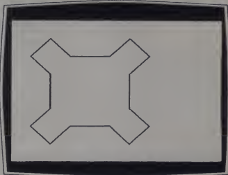
Figure 4. First order curve.
