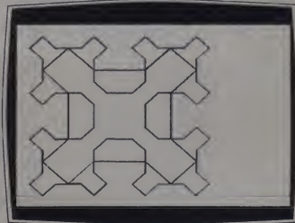
Figure 6. First and second order curves.
