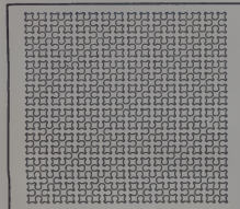
Figure 4. Sierpinski order 4.
