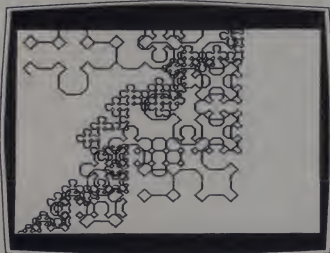
Figure 3. Curve with increased vertical height.
