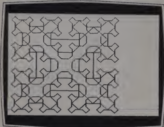
Figure 7. First to third order curves.
