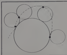
Figure 2. Generating an epicycloid.
