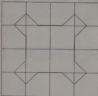
Figure 1. Geometric construction of first order curve.
