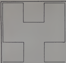
Figure 1. Hilbert order 2.
