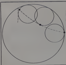
Figure 1. Generating a hypocycloid. July 1984 © Creative Computing
