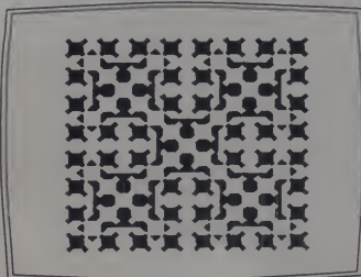
Figure 18. Second and fourth order curve painted from the center and outside.
