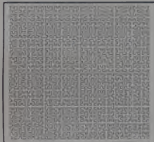
Figure 2. Hilbert order 6.
