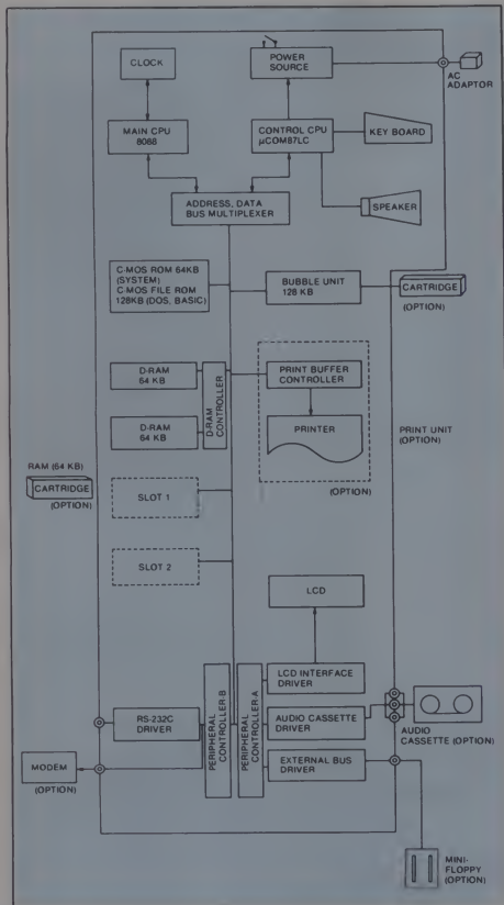
Figure 2. System block diagram of the PC-5000.
