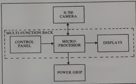
Figure 2. This unofficial block diagram of the Minolta X-700 Multi-Function Back shows how simple the accessory is, yet it operates in nine different control and imprint modes.
