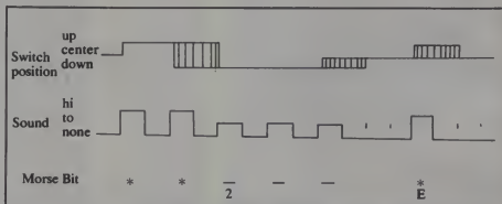
Figure 3. A switch position-sound correspondence timing diagram shows what sounds are produced by a certain switch motion and how the sounds generate Morse code. Note that precise timing of the sound intervals is not required of the operator and that reasonable timing uncertainties are allowable between the start of a high or low tone and its opposite.
