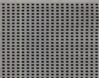
Figure 4. Multiplication mod 15: (0)yellow, (1)black, (2)yellow, (3)black, (4)yellow, (5)black, (6)yellow, (7)black, (8)yellow, (9)black, (10)yellow, (11)black, (12)yellow, (13)black, (14)yellow.
