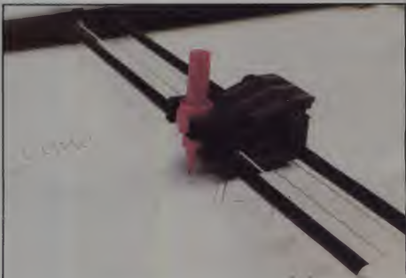
Pens move in step sizes of 0.001", 0.005", or 0.1 mm and at one of five different velocities.
