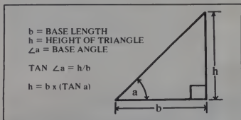
Figure 1. Relationships in a right triangle.
