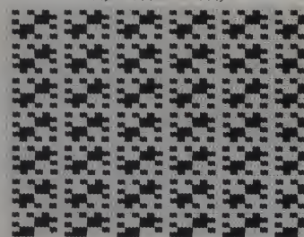
Figure 3. Multiplication mod 7: (0)yellow, (1)dark blue, (2)yellow, (3)dark blue, (4)yellow, (5)dark blue, (6)yellow.
