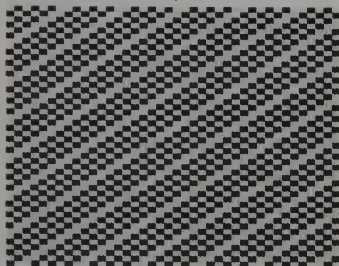
Figure 1. Addition mod 7: (0)yellow, (1)black, (2)yellow, (3)black, (4)yellow, (5)black, (6)yellow.
