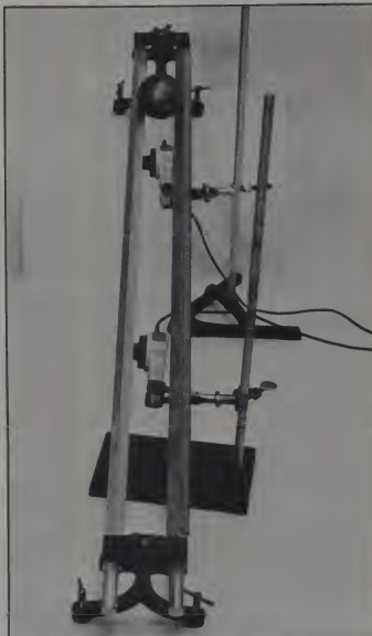
Photo 3. Only the paddle buttons are used in the velocity/acceleration timer. The ball must be heavy enough to activate them.
