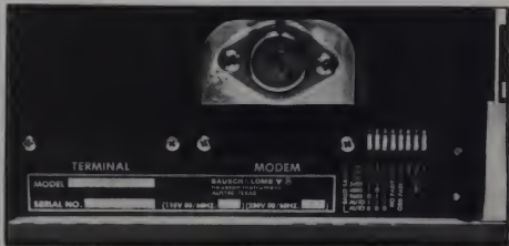
Plotter has RS-232 ports built in; Centronics and IEEE-488 ports are available as options. Up to 9600 baud can be set with the dip switches.
