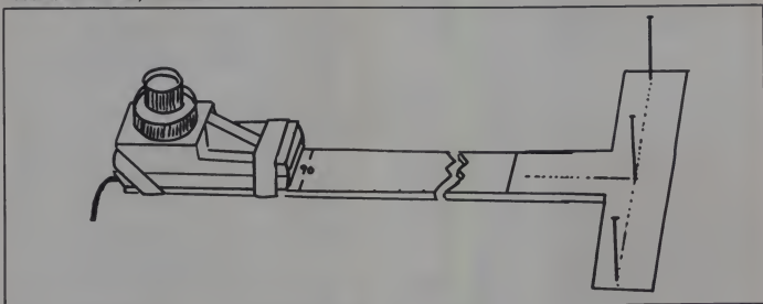
Figure 2. Rangefinder apparatus is constructed from a meter stick, cardboard "T", and game paddle.
