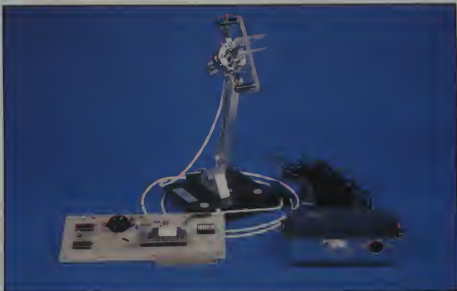
Figure 1. The center device is a Morse keyer mounted to be operated with up and down chin motion. It will drive both of the firmware implementations of the Serial Code Keyboard shown. The unit on the left is an Apple specific card which will operate from any I/O slot and sits electrically between the keyboard and the CPU board. The unit on the right is designed to operate with any dumb RS-232 type terminal.
