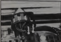
Dot matrix print element has a pair of wires leading to each of seven solenoids corresponding to seven striker pins.
