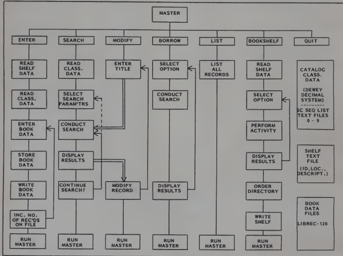
Figure 7. Structure of Library Catalog Program.
