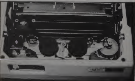
Some printer ribbons are in easy-to-change cartridges. Others use typewriter-like spools that are more difficult to change.
