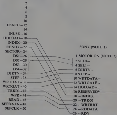
Figure 3. Adapter configuration.
