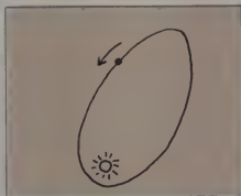
Figure 6. A highly elliptical orbit leading to hot summers and cold winters.
