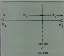
Figure 3. Bringing the center of mass to the center of the screen.
