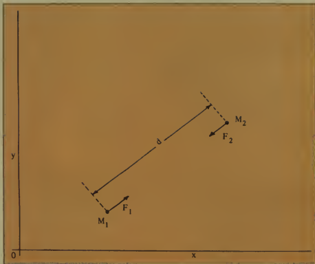
Figure 1. Two bodies in the x-y plane.
