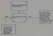
Figure 2. Defensive flow-chart.
