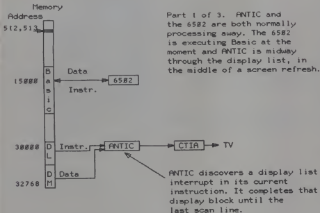
Diagram 2, part 1 of 3. Display List Interrupt Processing.
