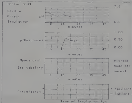
Figure 4. Graphic summary of arrest simulation. This summary is a different simulation than the other example figures.
