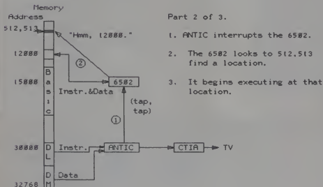
Diagram 2, part 2 of 3. Display List Interrupt Processing.
