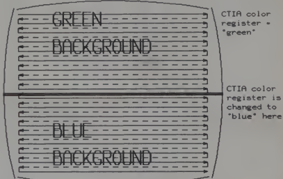
Diagram 1. One TV refresh (this process happens 60 times/sec).
