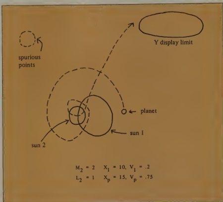
Figure 10. An unstable orbit.
