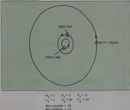
Figure 8. A stable orbit around both suns.
