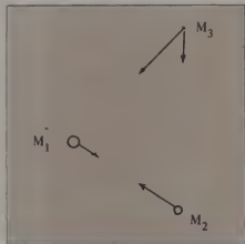
Figure 4. The two suns attract the planet and each other.
