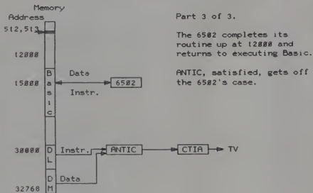
Diagram 3. Storing an assembly program as a string.
