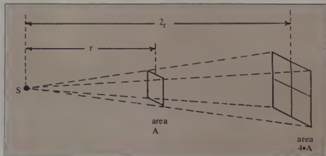
Figure 7. The interception of energy radiated from S.
