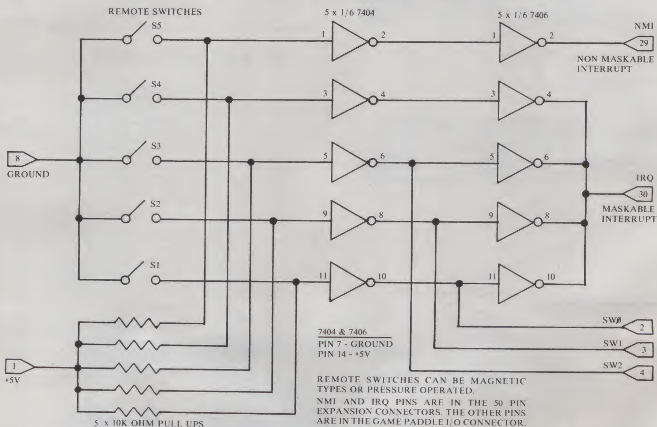
Figure 3. Interrupt Control Circuit.
