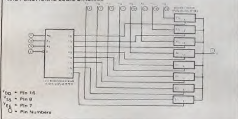
4051B FUNCTIONAL LOGIC DIAGRAM
