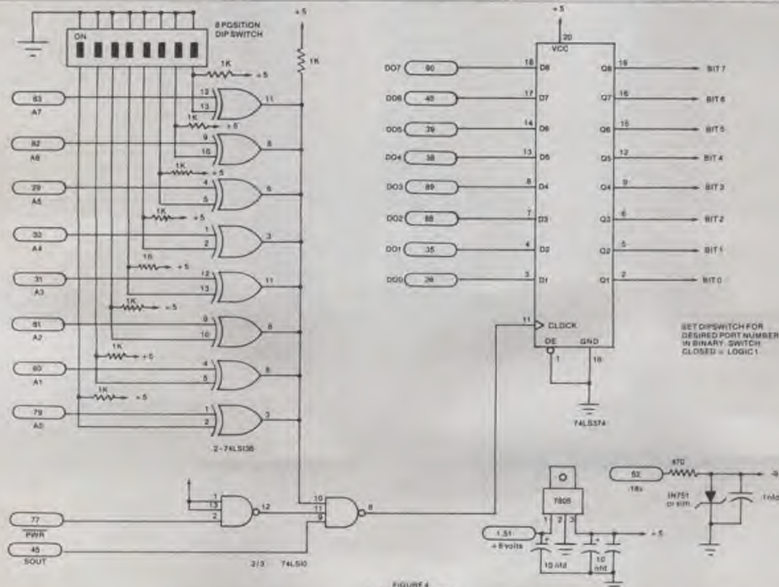
FIGURE 4 5-1 DI PARALLEL PORT
