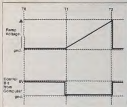
Figure 2. Timing diagram of control bit from computer and ramp from A/D converter.
