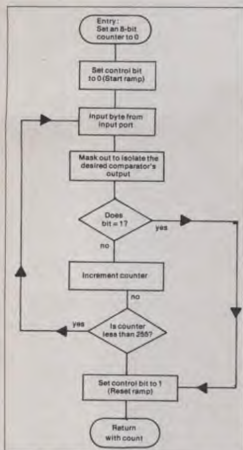
Figure 5. Flowchart of a machine language conversion program.
