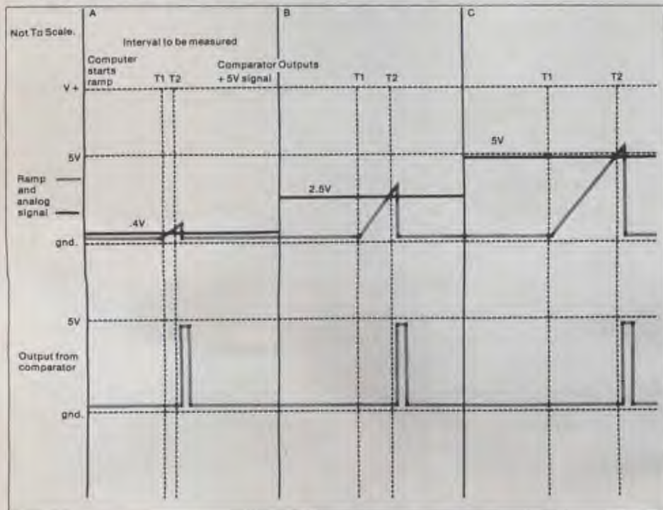
Figure 3. Timing diagram of ramp, analog input and output from comparator.
