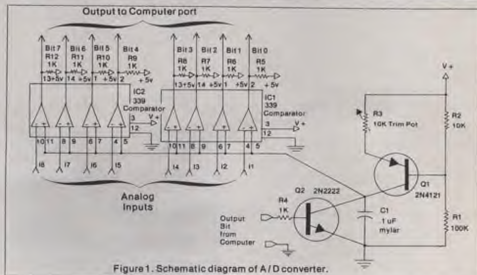
Figure 1. Schematic diagram of A/D converter.
