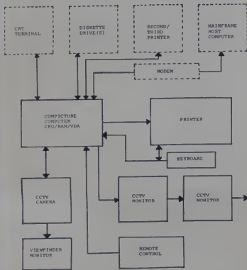
Figure 1. The CPU (Central Processing Unit) is a 5-100 bus micro-computer with 2 serial I/O and 2 parallel I/O ports. Size of RAM varies from system to system. Dotted items across the top are optional.
