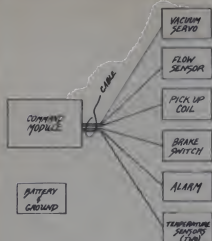
Figure 1. A block diagram of the Compucruise System. All interconnecting wires are color coded and they end in snap-on connectors.
