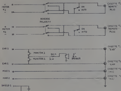
[FIG 2] Schematic diagram of the auxiliary cassette tape recorder controls
