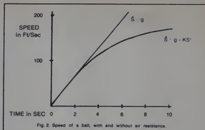
Fig. 2. Speed of a ball, with and without air resistance.
