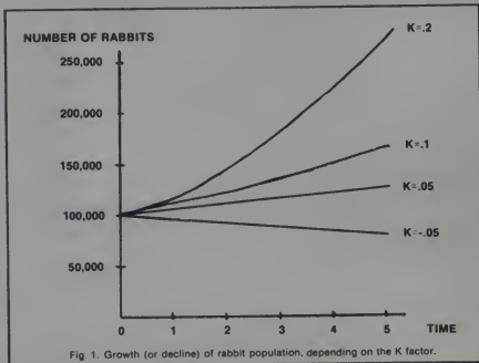
Fig. 1. Growth (or decline) of rabbit population, depending on the K factor.
