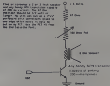
FIGURE 4 SELF-CONTAINED PET SOUND/HAKE CIRCUIT
