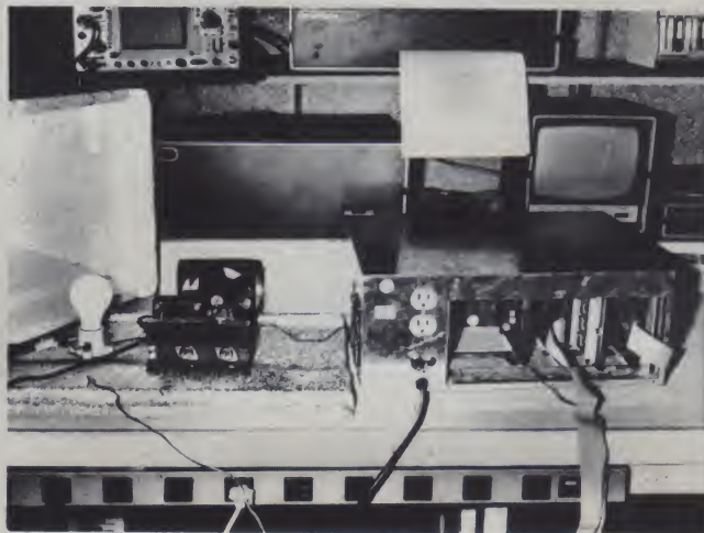
This lab set-up uses the Real World Interface and a temperature probe to control how long the lightbulb stays on, so as to cycle the temperature up and down at a predetermined rate. The printer output is at top.
