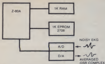
Fig. 4A. The Cromemco Z-1 system as used for EKG processing.
