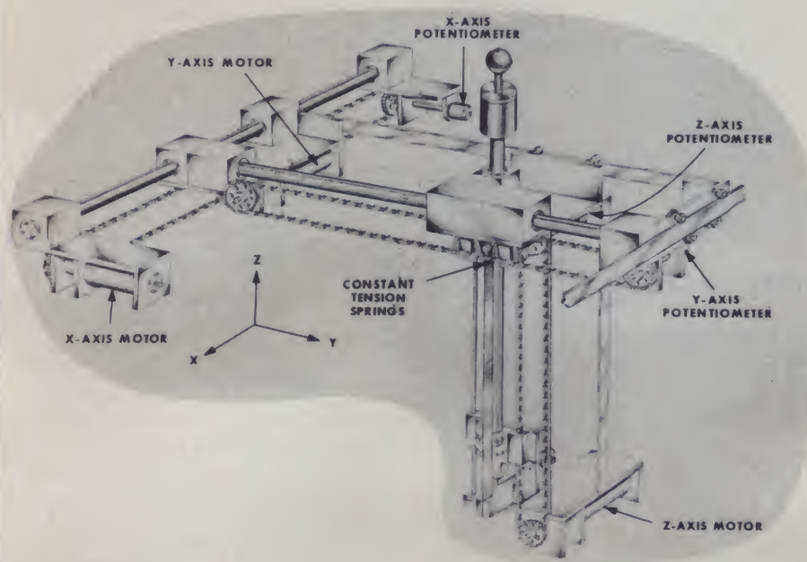
Fig. 1. Sketch of tactile device. The ball at the top of the vertical shaft can be moved within a 10-inch cubical space. The position of the ball is sensed by potentiometers while the force required to move the ball is controlled by motors.
