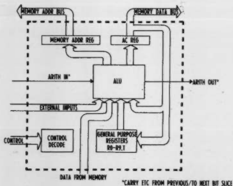
FIGURE 3a: INTEL 3002 CENTRAL PROCESSING ELEMENT (2-BIT SLICE)
