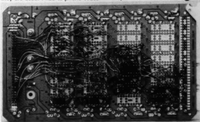
Rear view: Dual Serial Interface
