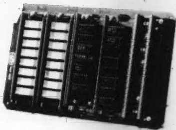
Front (top) view: 8K Dynamic Memory Module
