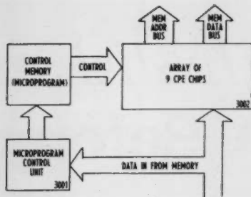
FIGURE 3b: INTEL 3000 SERIES CONFIGURED AS 18-BIT CPU
