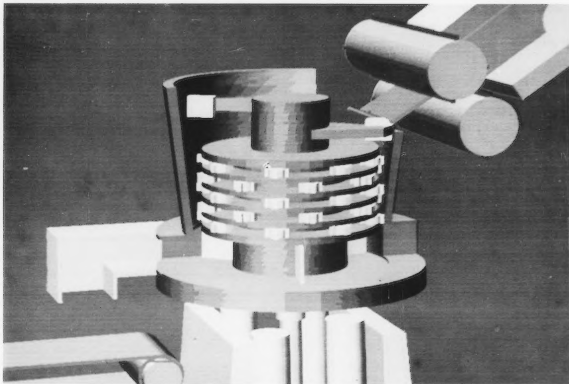
The function of this machine is to chew whole cars into pieces about the size of a quarter. Obviously the process cannot be photographed from the inside, but Synthavision showed in a representational fashion how it works.
