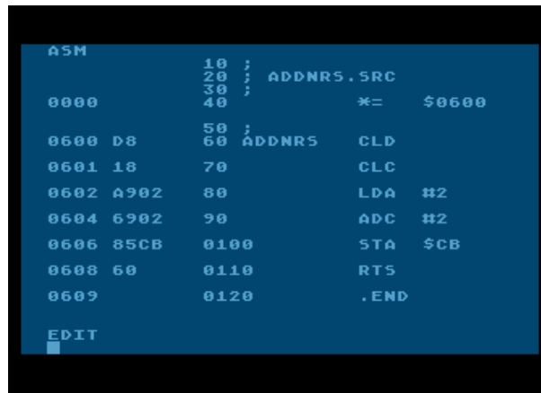
Screen Shot Of ADDNRS.SRC
