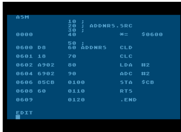
Screen Shot Of ADDNRS.SRC Assembled With The Atari Assembler Editor
